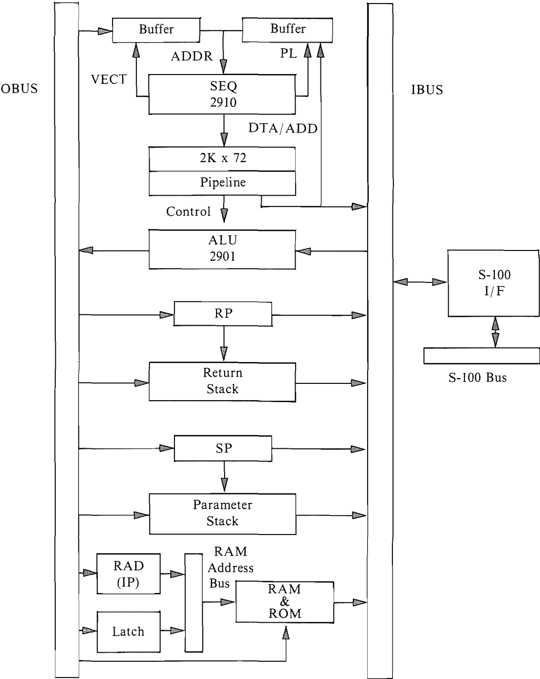
Figure 1. The System Block Diagram of RUFOR.
