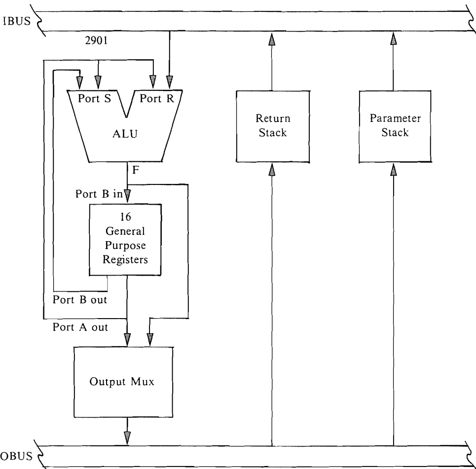
Figure 2. The ALU Flow Diagram
