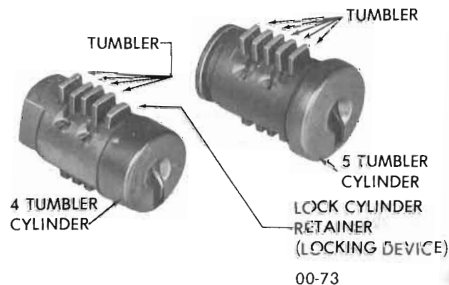
Figure 00-8 - Glove Compartment Lock Cylinder
