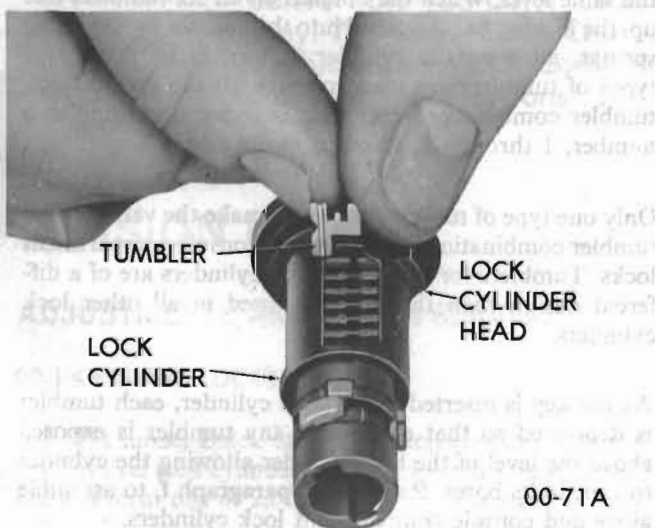
Figure 00-2 - Installing Tumblers
