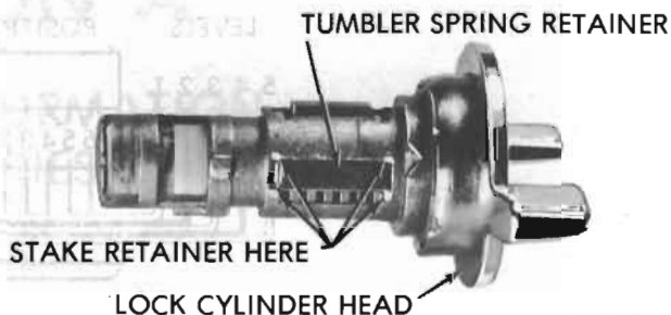
Figure 00-3 - Installing Spring Retainer
