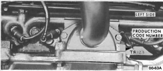
Figure 00-13 - Engine Serial Number and Production Code Location (455 Cu.In.)
