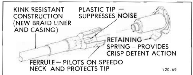
Figure 120-69 Quick Connect Speedo Cable
