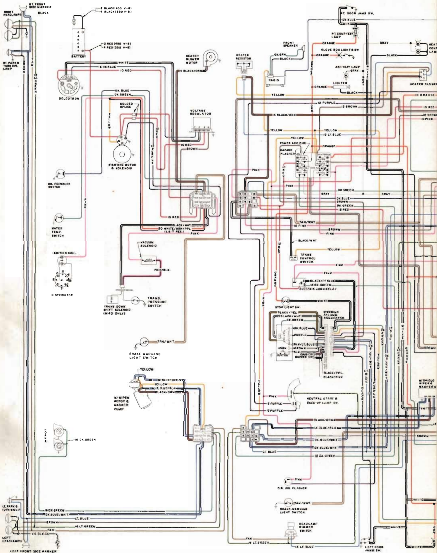
Figure 120-133 Wiring Circuit Diagram - 43-44000 Series
