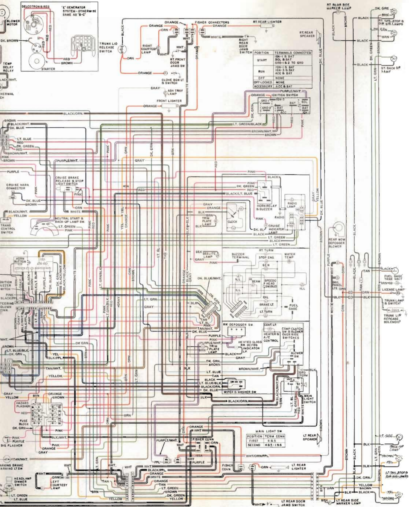
Diagram - 45-46-48-49000 Series
