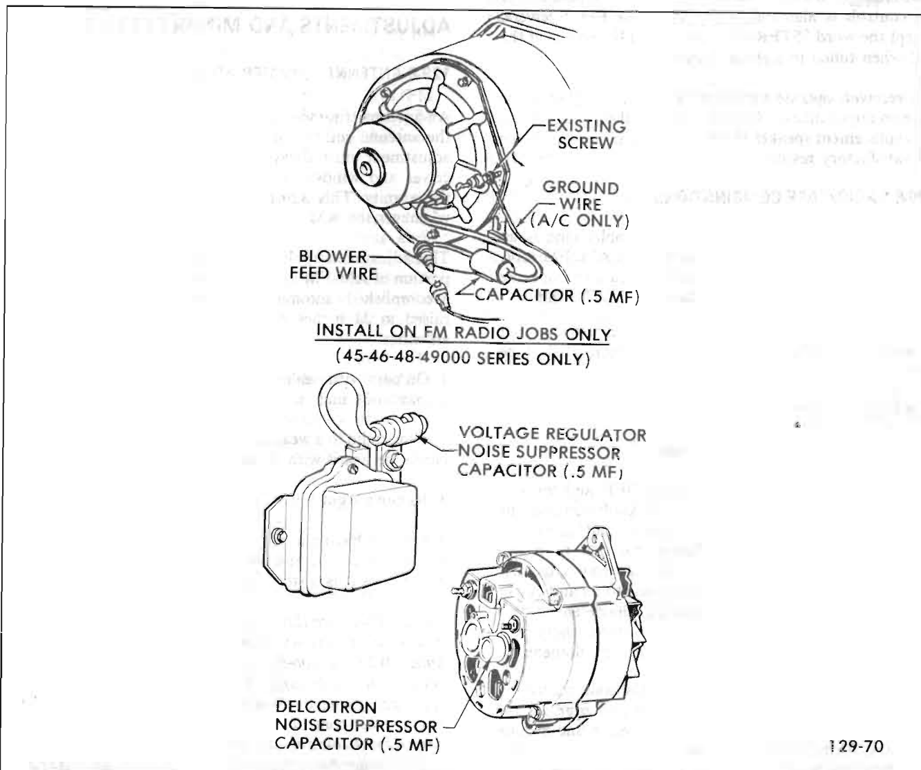
Figure 129-1 - Installation of Noise Suppressors
